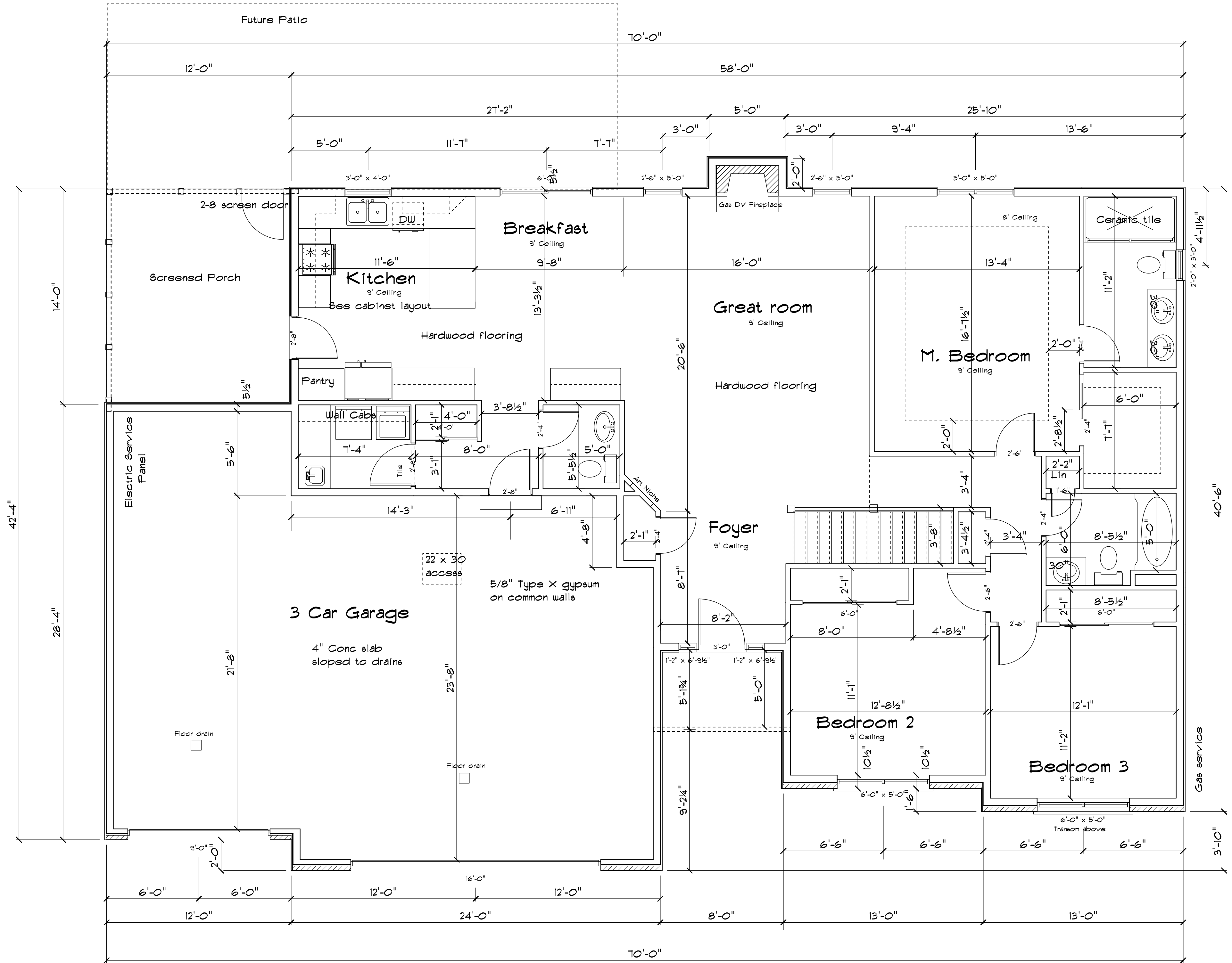
Main Floor Plan Scale 1/4" = 1'0" 1767 SF
