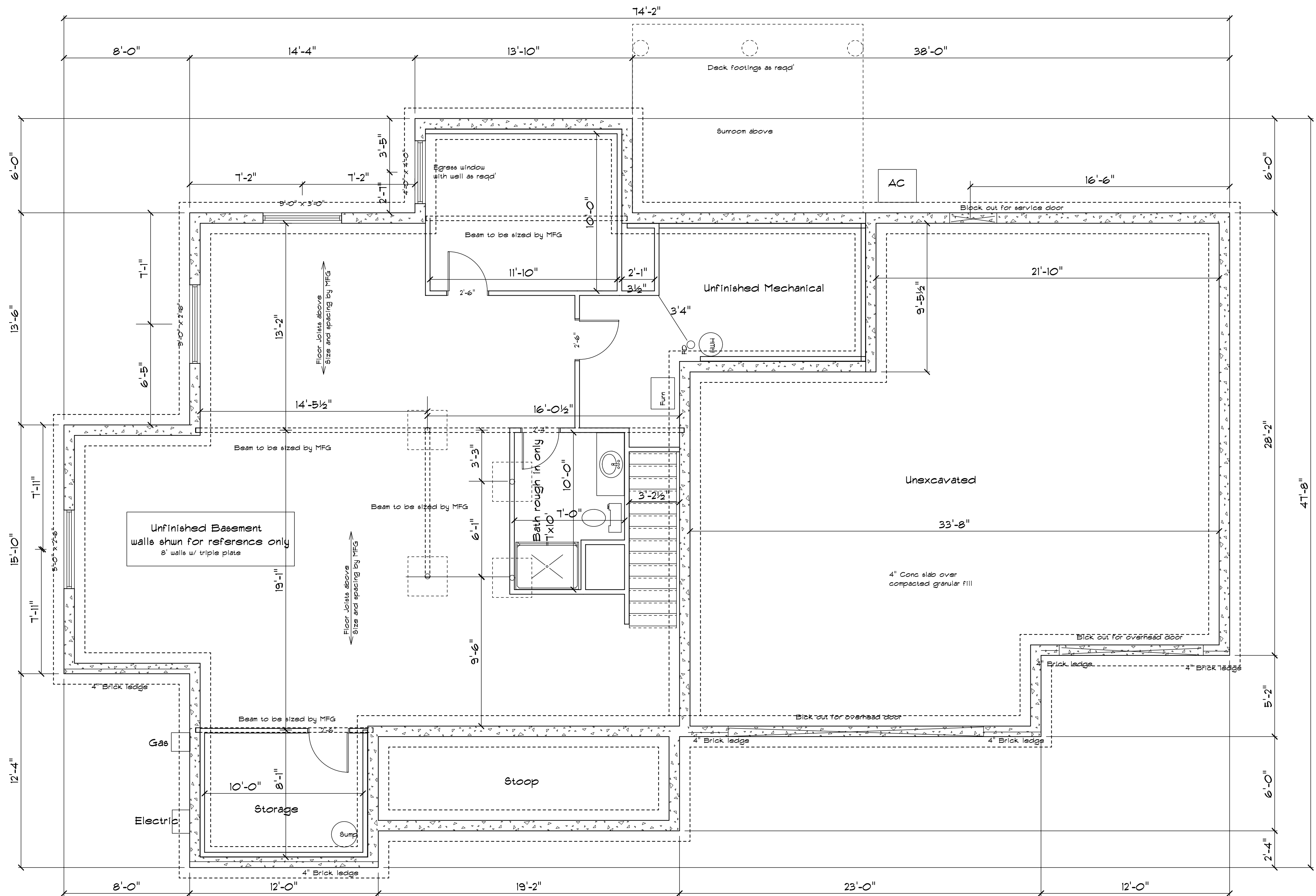
Foundation Plan
