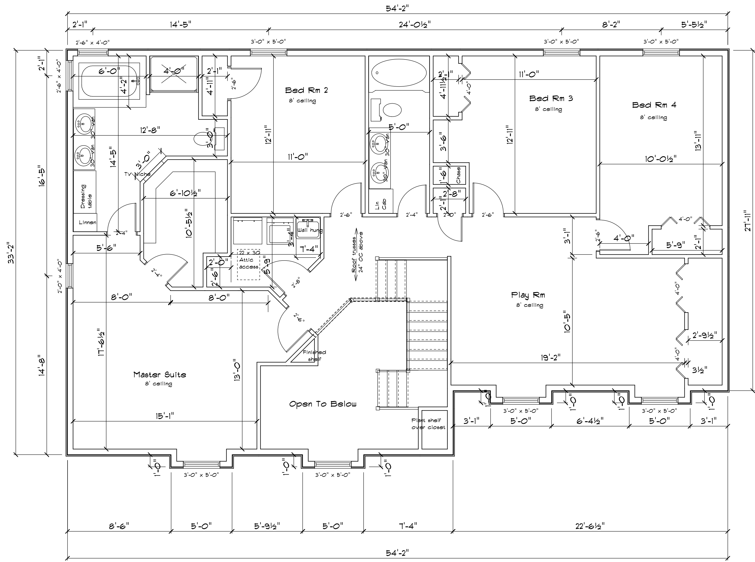
Second Floor Plan 1500 SF
