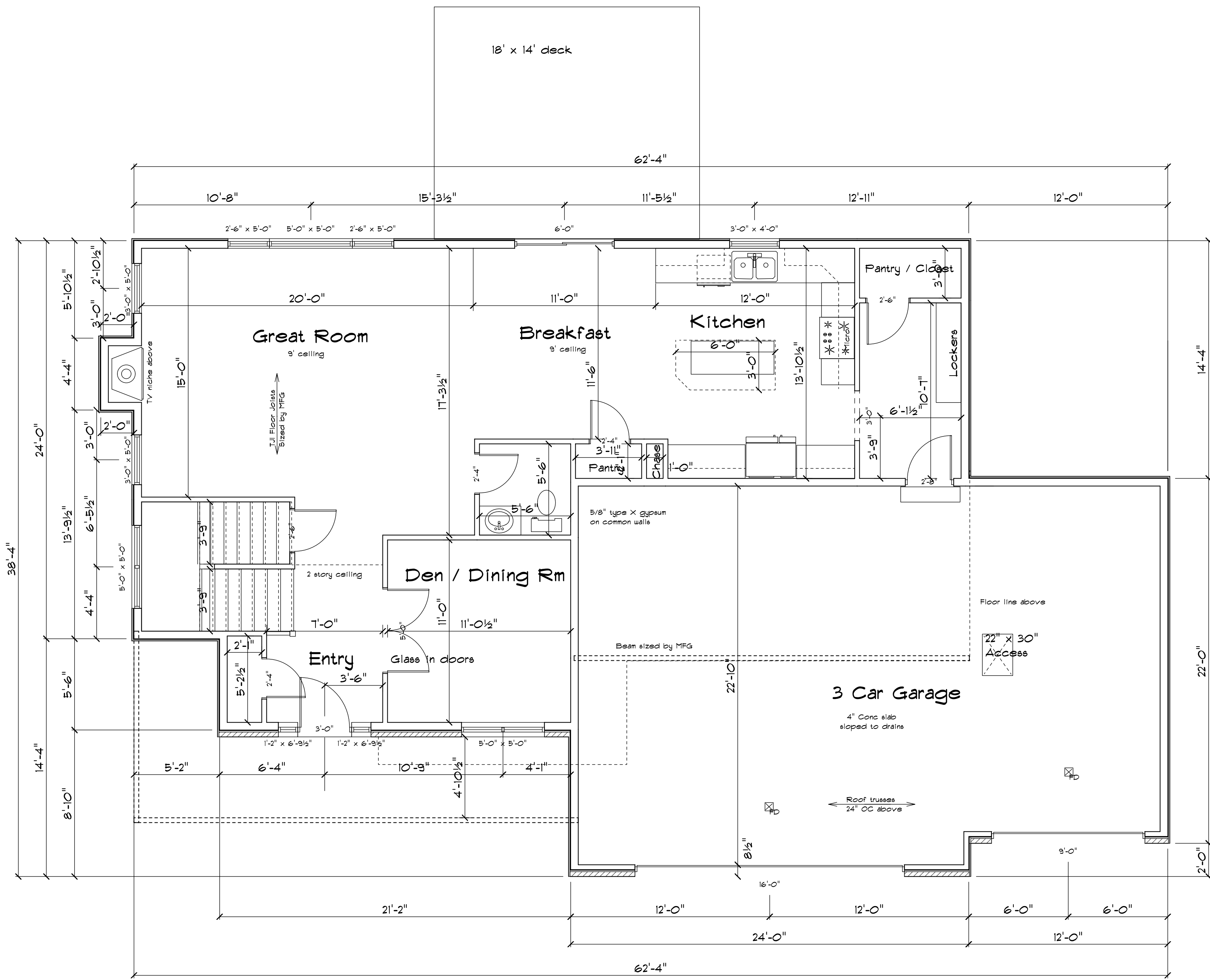
Fairview First Floor 1122 SF
