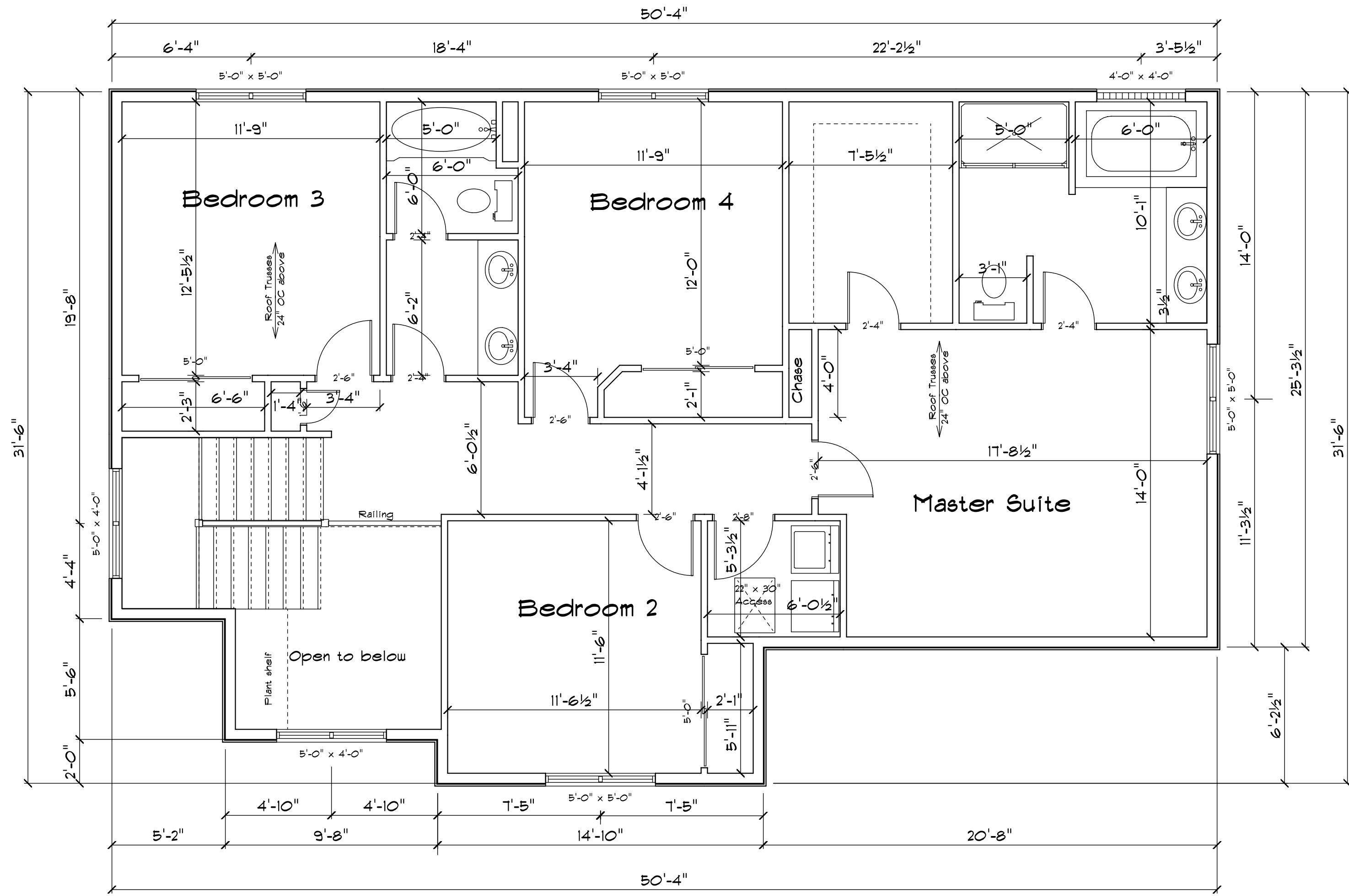
Fairview Second Floor 1262 SF
